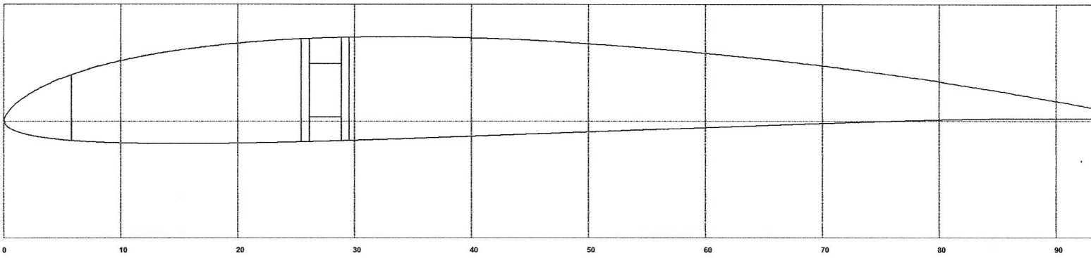
RIB 4 Chord (millimetres) : 219.000 L.E. Ref. Distance (millimetres) : 21.000 C.L. Ref. Distance (millimetres) : 187.500
