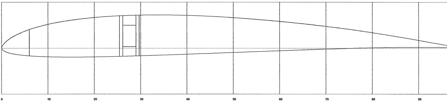
RIB 5 Chord (millimetres) : 212.000 L.E. Ref. Distance (millimetres) : 28.000 C.L. Ref. Distance (millimetres) : 234.375
