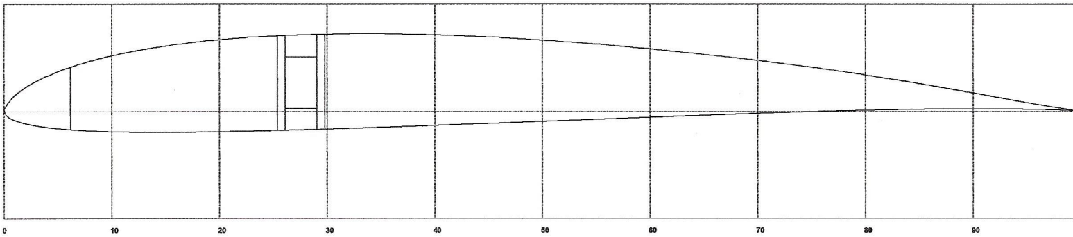
RIB 6 Chord (millimetres) : 205.000 L.E. Ref. Distance (millimetres) : 35.000 C.L. Ref. Distance (millimetres) : 281.250
