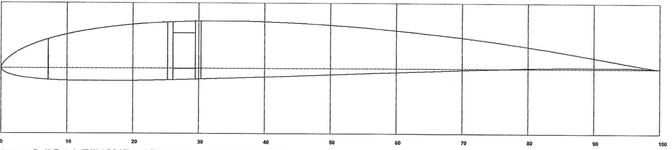
RIB 10 Chord (millimetres) : 177.000 L.E. Ref. Distance (millimetres) : 63.000 C.L. Ref. Distance (millimetres) : 468.750
