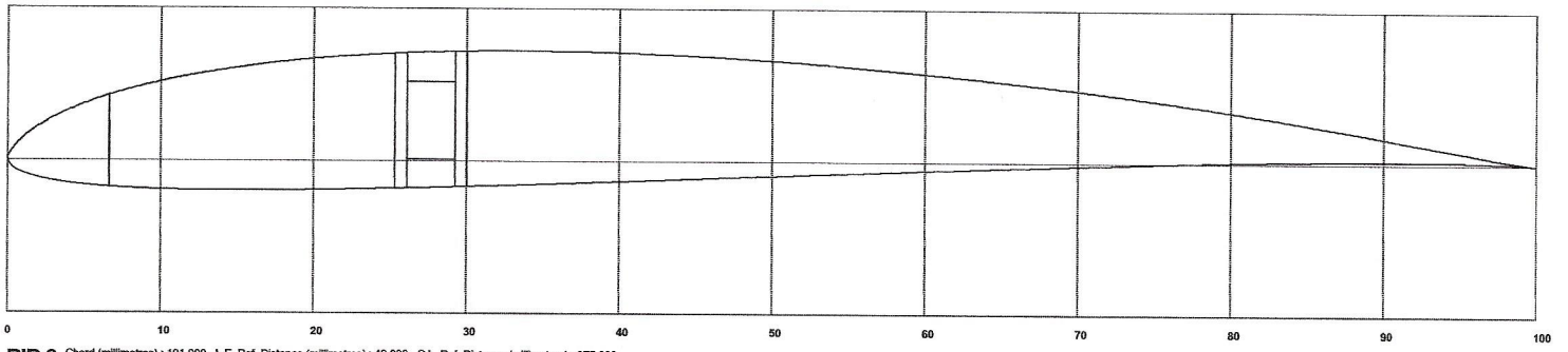
RIB 8 Chord (millimetres) : 191.000 L.E. Ref. Distance (millimetres) : 49.000 C.L. Ref. Distance (millimetres) : 375.000
