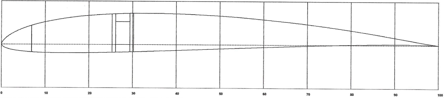
RIB 9 Chord (millimetres) : 184.000 L.E. Ref. Distance (millimetres) : 56.000 C.L. Ref. Distance (millimetres) : 421.875
