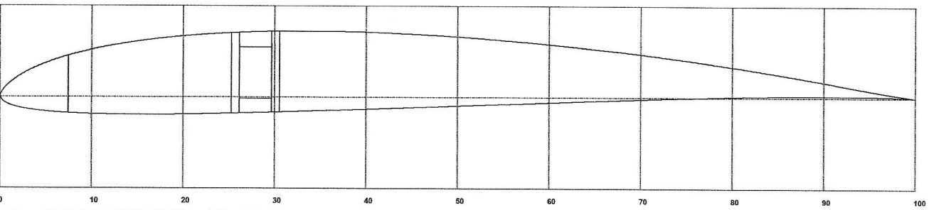
RIB 11 Chord (millimetres) : 170.000 L.E. Ref. Distance (millimetres) : 70.000 C.L. Ref. Distance (millimetres) : 515.625
